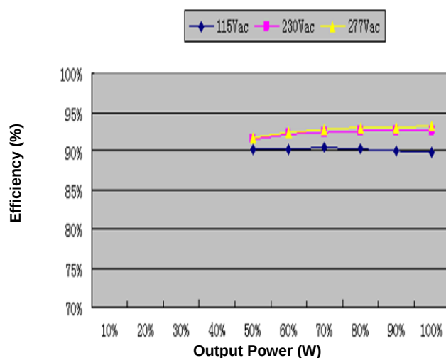
Figure 2: Efficiency vs. Output Power (Vo=24V)
